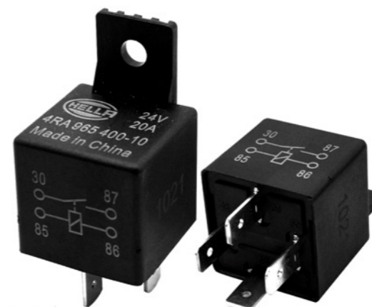
ELF036 RELAY HELLA 4 PATAS 20 AMP 24V X1
